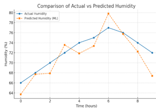
Figure 8. Comparison of Actual Humidity with Machine Learning
